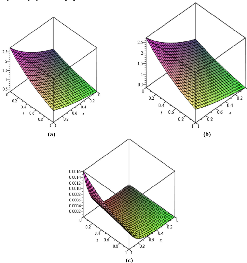
Fig. 1 The surface shows the solution u(x, t) for equations (22)-(24) when
