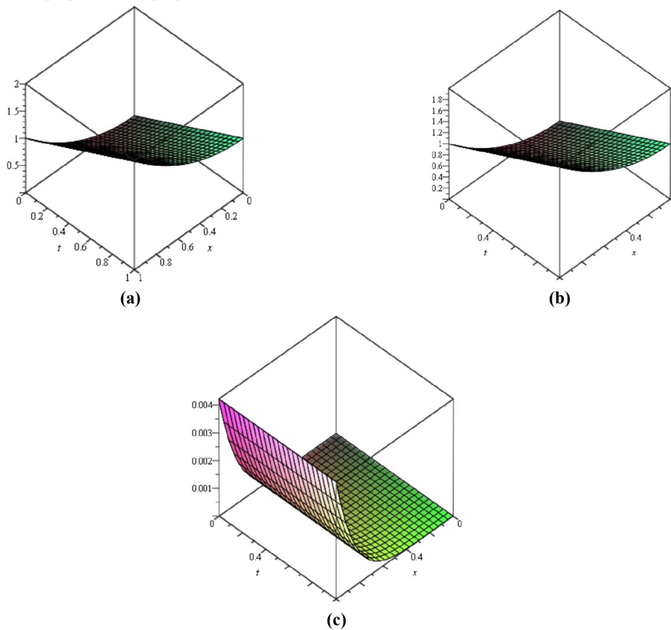
Fig. 3 The surface shows the solution u(x, t) for equations (33)-(35) when
