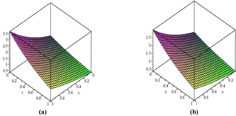
Fig. 2 The surface shows the solution u(x, t) for equations (22)-(24):
